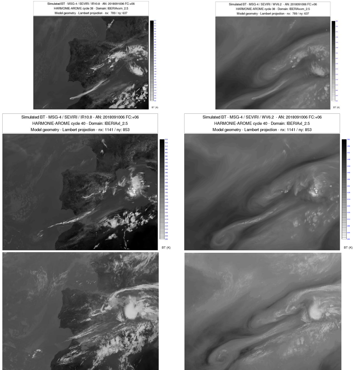
Figure 4: IR10.8 (left) ad WV6.2 (right) images from an experiment based on cycle 38 of HARMONIE-AROME (top), from an experiment based on cycle 40 (middle) and observed Meteosat-11 (bottom), all for 20180910 at 12 UTC.
