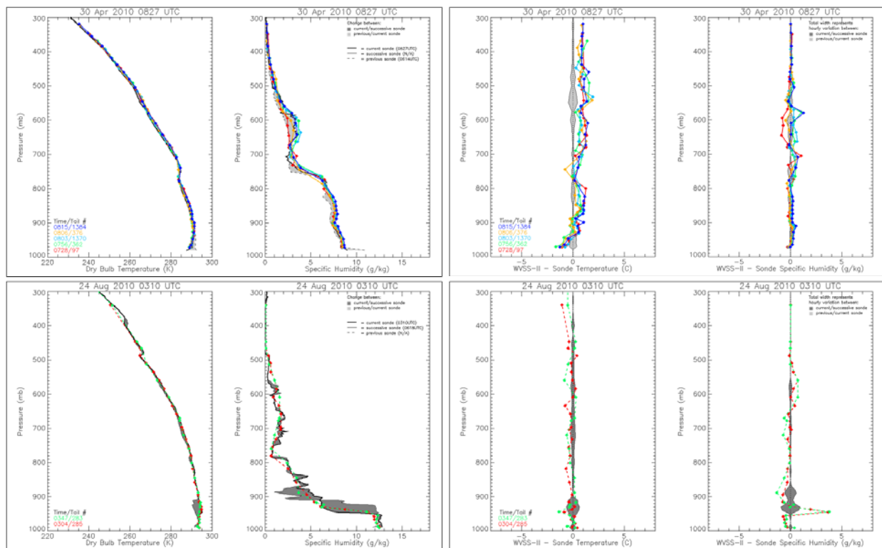
Figure 3 - Top Left - Plots of co-located ascending WVSS-II observations (colored) and rawinsonde data (black) taken around 0827 UTC on 30 April 2010 at Rockford IL. Temperature (C) at left, Specific Humidity (g/kg) at right, solid lines during descent, dashed lines during ascent. Changes between bounding rawinsondes shaded. Top Right - Differences between rawinsonde and ascending aircraft observations using same color convention as top panel. Shading indicates \pm 50\% of hourly changes observed between bounding rawinsonde reports. Bottom - Same as top panels, except for descending WVSS-II observations taken around 0310 UTC on 24 August 2010.
