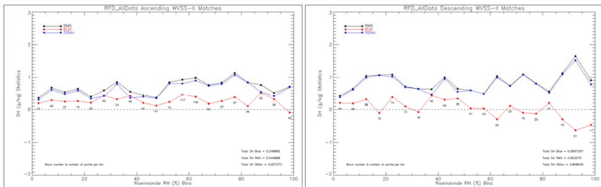
Figure 5 - Comparison of systematic (Bias) and random (StDev) differences in WVSS-II SH observations during all intercomparison periods at different 5% RH ranges for ascending (left) and descending (right) aircraft.
