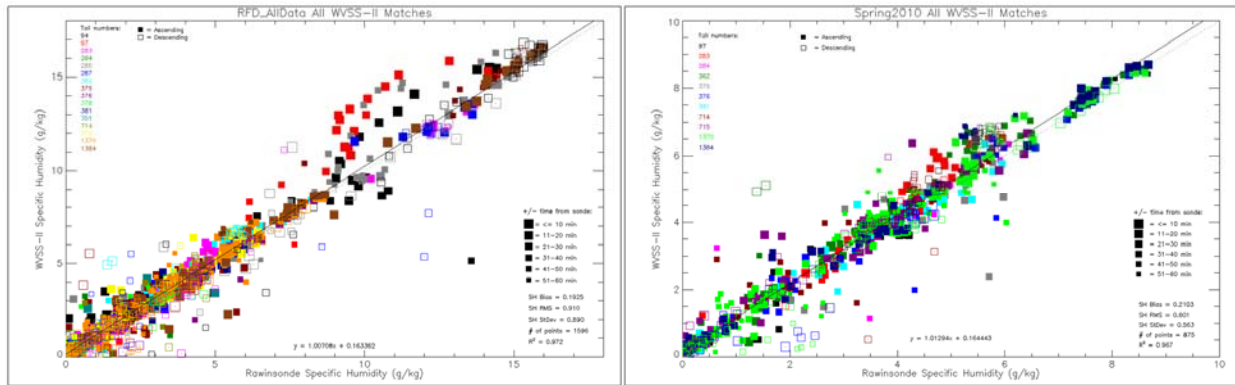
Figure 4 - Scatter plot showing inter-comparison of WVSS-II and co-located rawinsonde Specific Humidity reports for all levels for all observation intercomparison periods (left) and period from 27 April-10 May 2010 at Rockford, IL. . Color coded by aircraft. Marker size indicates time spread between WVSS-II and rawinsonde observations – larger markers indicate matchups that are closer in time. Ascents presented as solid squares, descents by open squares. Statistics included in lower right.
