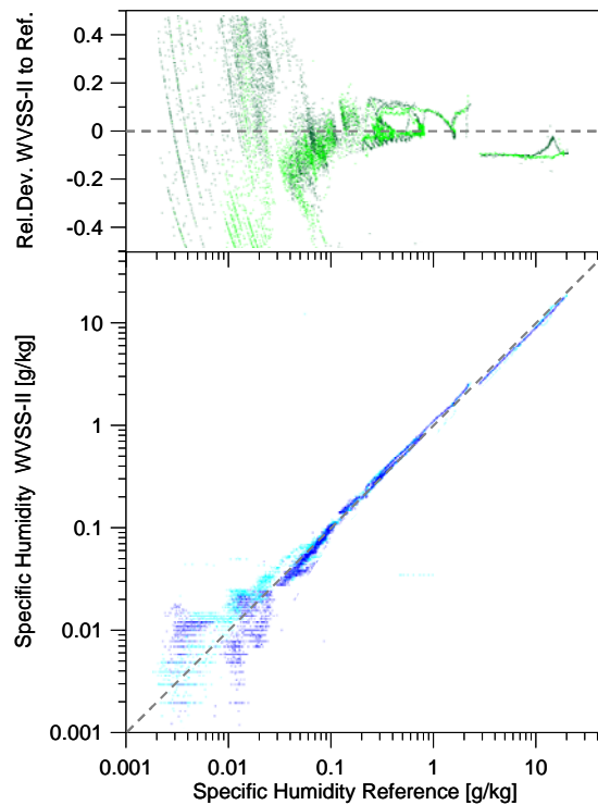
Figure 2 - Comparison of WVSS-II versus Lyman (a) fluorescence hygrometer (0.001 - 1 g/kg) and dew / frost point hygrometer (General Eastern, Type D1311R, 1 - 40 g / kg) obtained from 2 simulation runs made in the FZJ climate chamber ( http://www.fz-juelich.de/icg/icg-ii/esf ) in July 2010.
