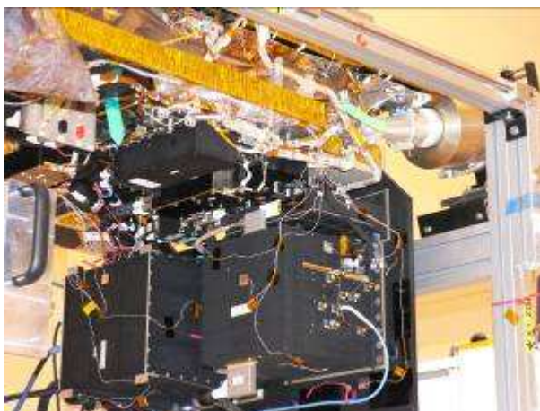
Figure 4 : SARAL/AltiKa Instrument
