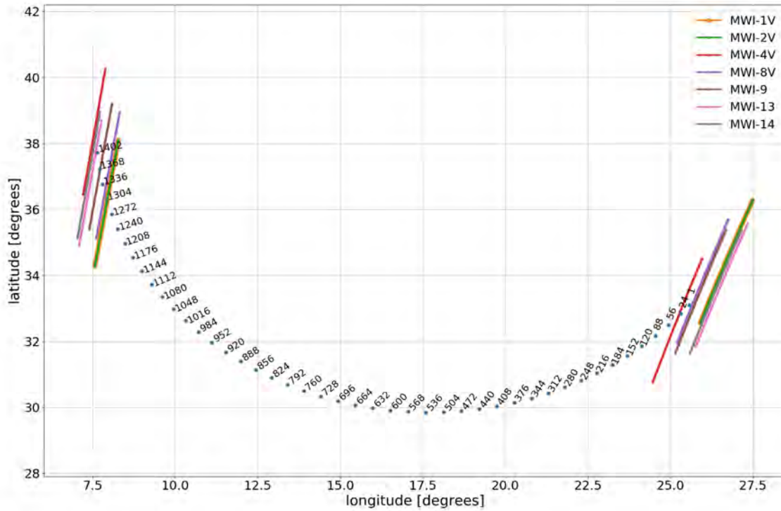
Figure 42: Geolocation on geoid of different sample positions for MWI-3V (target channel) within a given scan. Geolocation of outer sample positions for neighboring scans and for some other MWI channels are also displayed. The figure indicate that it should be possible to remap observations for all channels for sample numbers between about 30 to 1300 (see Table 8 for actual range and corresponding scan angles).
