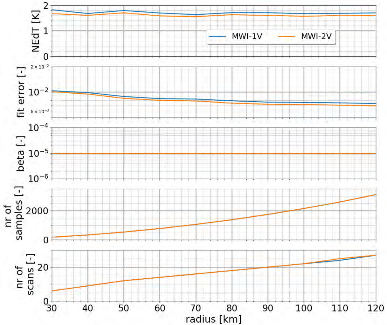
Figure 45: As Figure 43 but for MWI-1V and MWI-2V. See text for more details.
