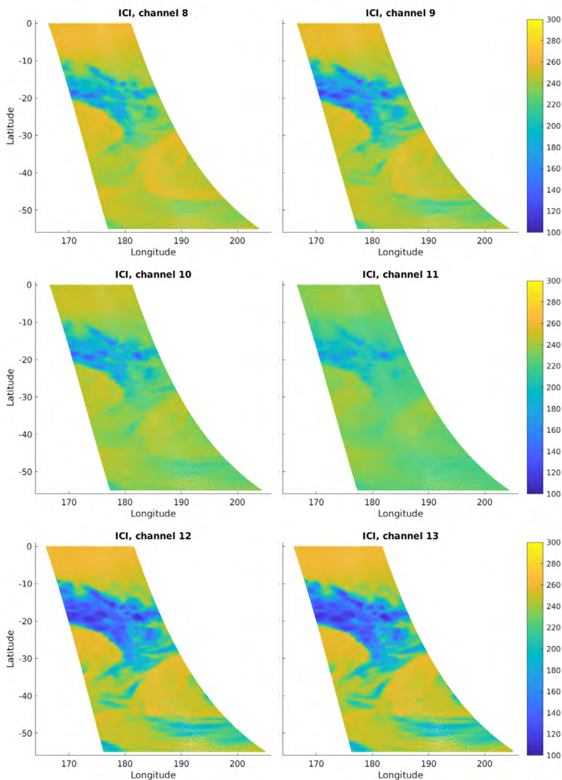
Figure 20: ICI simulations for channel 8-13 and same part of orbit 6895 as shown in two previous figures.
