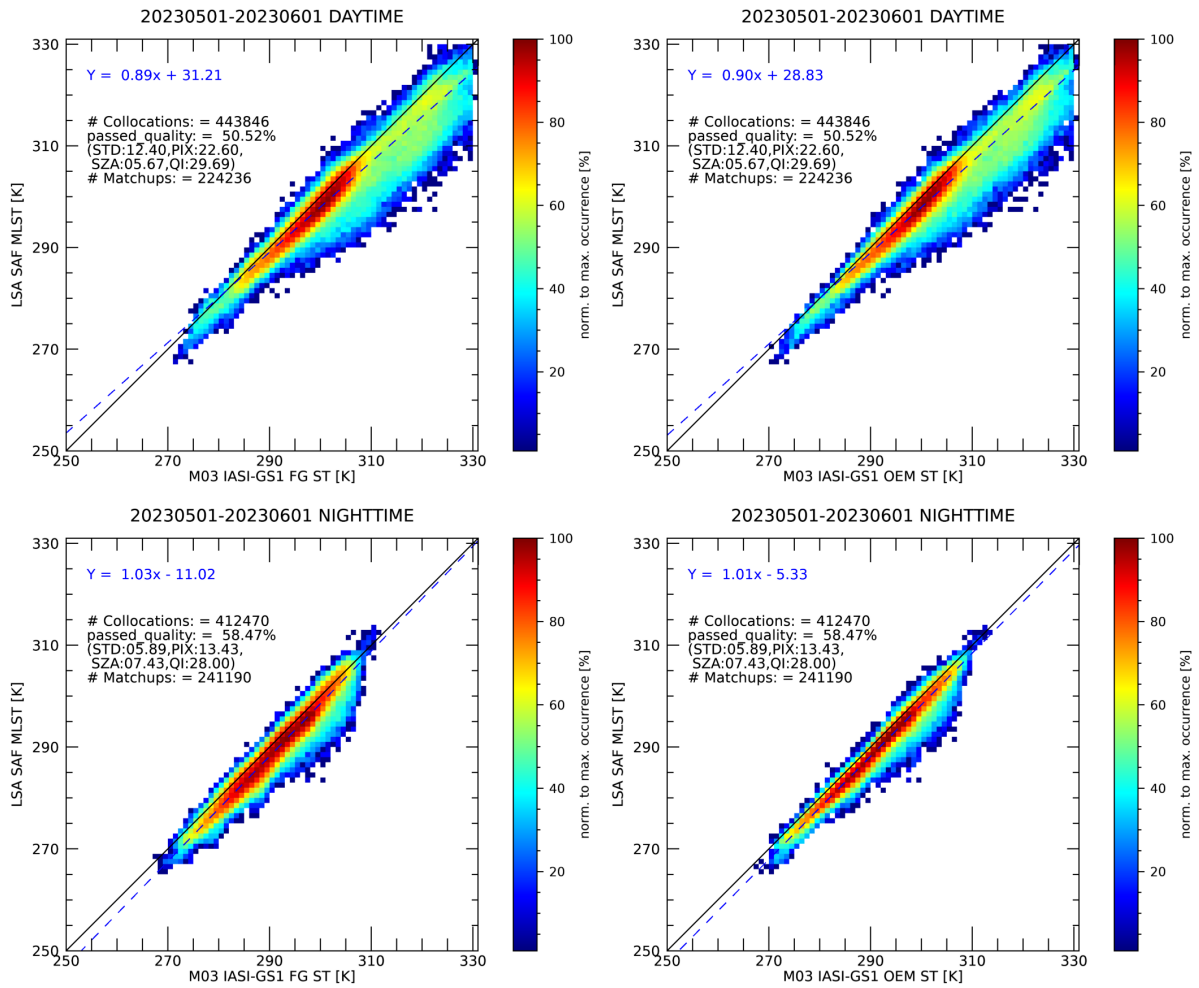
Figure 3.6: 2D Histograms for Day (top), Night (Bottom), Regression (FG) (left) and OEM (right) retrieval, with M03 IASI L2 from GS1 for 01-31/05/2023
