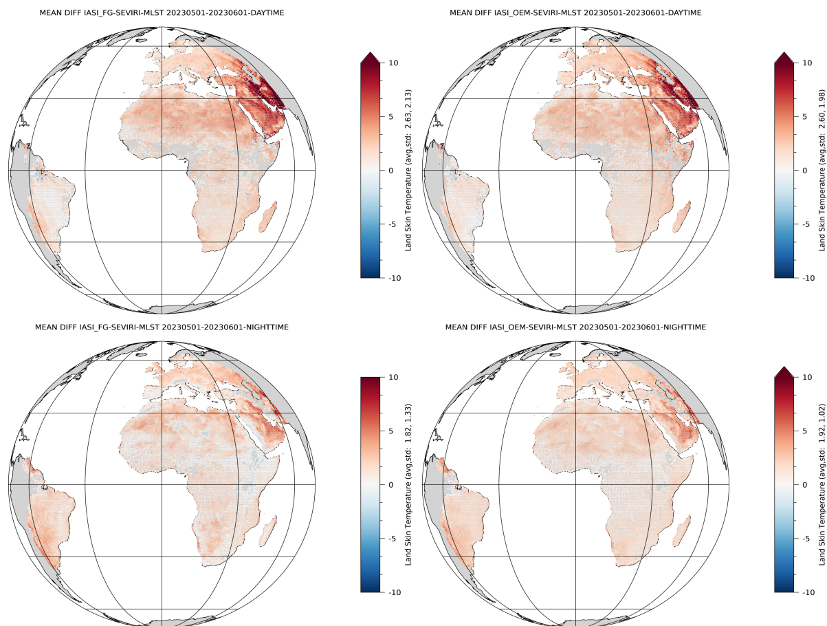
Figure 4.1: Day (top) and Night (bottom) Maps with mean Differences of the differences IASI - LSA SAF for Regression (FG) (left) and OEM (right) retrieval, with M03 IASI L2 from GS1 for 01-31/05/2023
