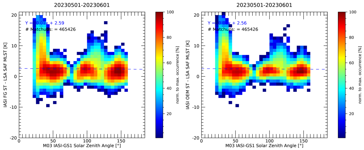
Figure 3.13: 2D Histograms difference of IASI - LSA SAF dependent on Solar Zenith Angle for Day (top), Night (Bottom), Regression (FG) (left) and OEM (right) retrieval, with M03 IASI L2 from GS1 for 01-31/05/2023
