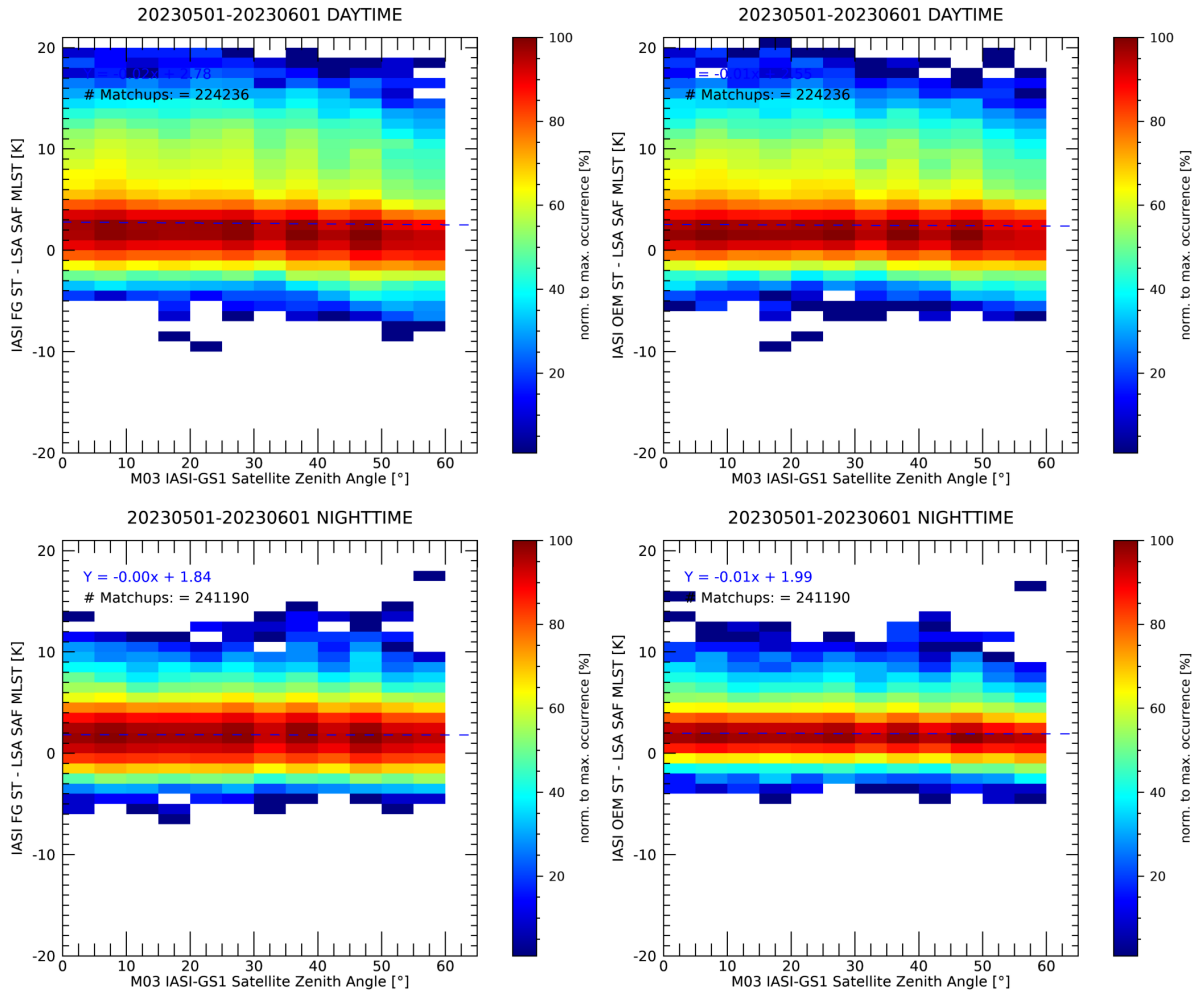
Figure 3.11: 2D Histograms difference of IASI - LSA SAF dependent on IASI Satellite Zenith Angles for Day (top), Night (Bottom), Regression (FG) (left) and OEM (right) retrieval, with M03 IASI L2 from GS1 for 01-31/05/2023
