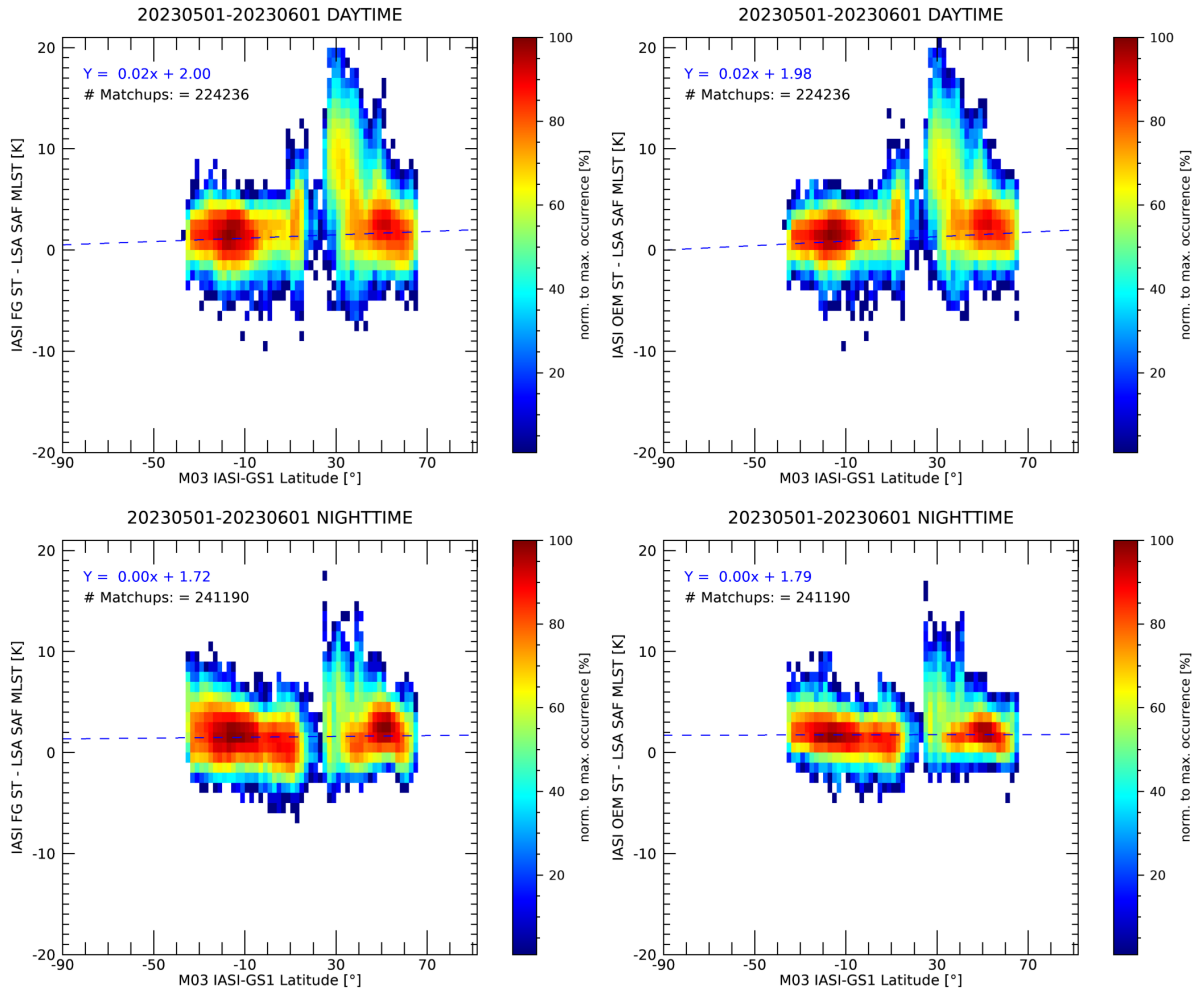
Figure 3.10: 2D Histograms difference of IASI - LSA SAF dependent on Latitude for Day (top), Night (Bottom), Regression (FG) (left) and OEM (right) retrieval, with M03 IASI L2 from GS1 for 01-31/05/2023
