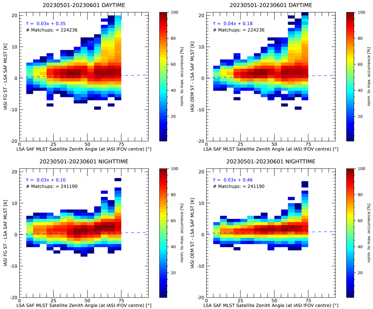
Figure 3.12: 2D Histograms difference of IASI - LSA SAF dependent on SEVIRI Satellite Zenith Angles for Day (top), Night (Bottom), Regression (FG) (left) and OEM (right) retrieval, with M03 IASI L2 from GS1 for 01-31/05/2023
