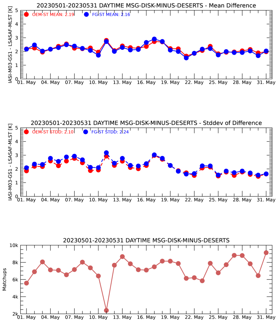
Figure 3.1: Monthly time series of mean difference and standard deviation between IASI L2 - LSA SAF. The bottom panel shows the number of daily match-ups. Daytime statistics with M03 IASI L2 from GS1 for 01-31/05/2023
