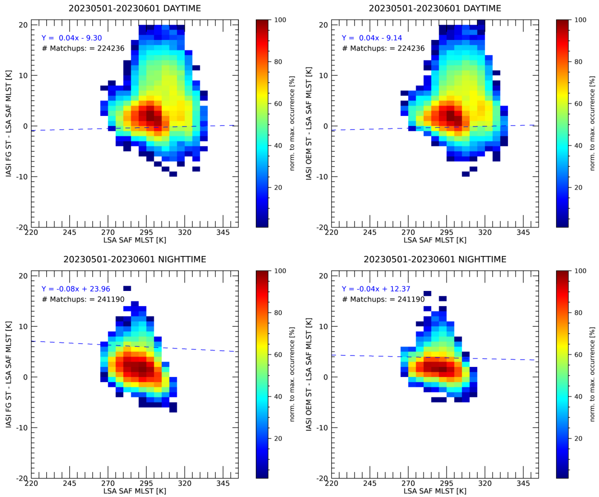
Figure 3.9: 2D Histograms difference of IASI - LSA SAF dependent on LSA SAF MLST for Day (top), Night (Bottom), Regression (FG) (left) and OEM (right) retrieval, with M03 IASI L2 from GS1 for 01-31/05/2023
