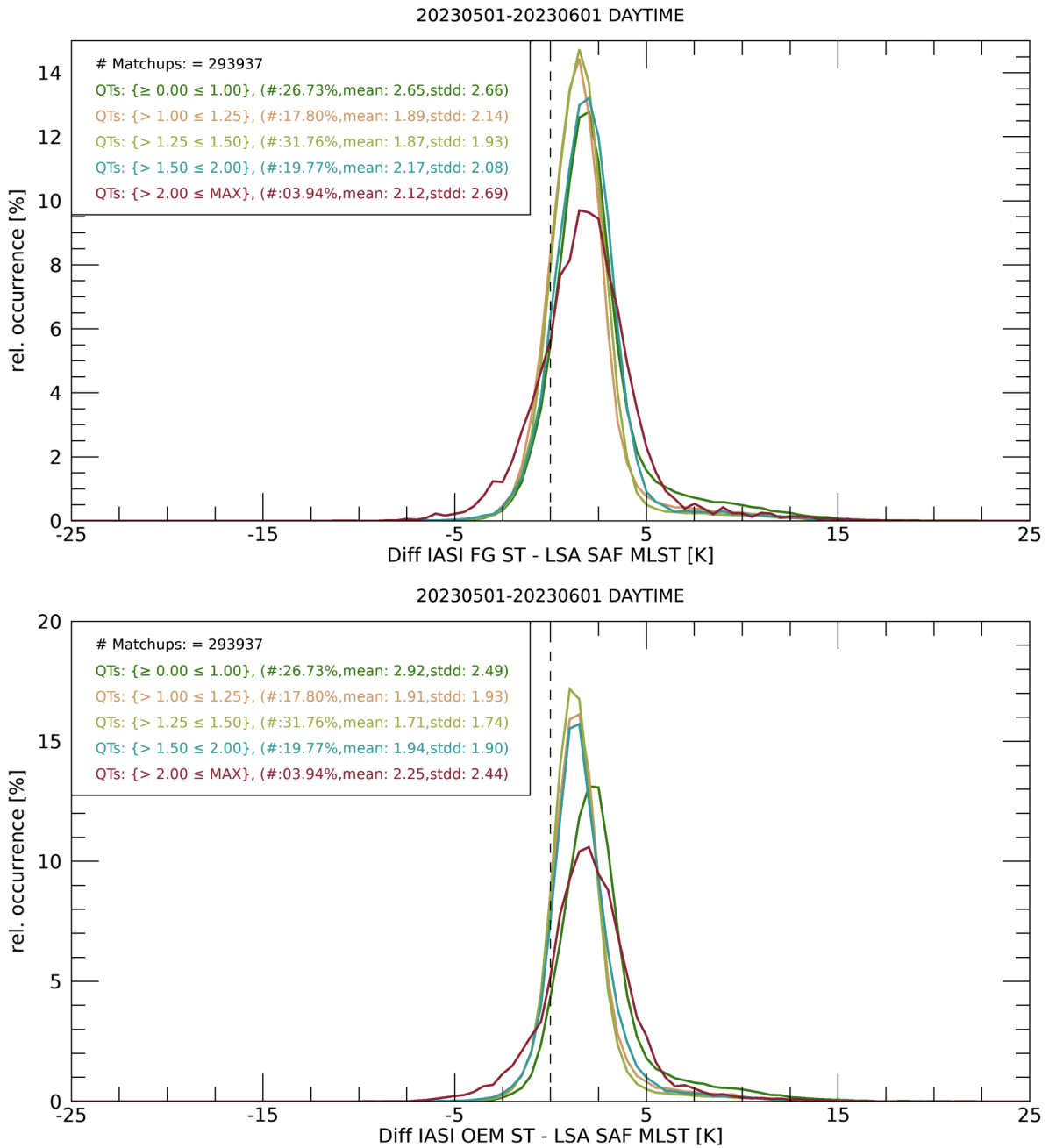
Figure 3.7: Difference histograms grouped for different quality indicators for Regression (FG) (top) and OEM retrieval (bottom) retrieval between IASI L2 - LSA SAF, Daytime statistics with M03 IASI L2 from GS1 for 01-31/05/2023
