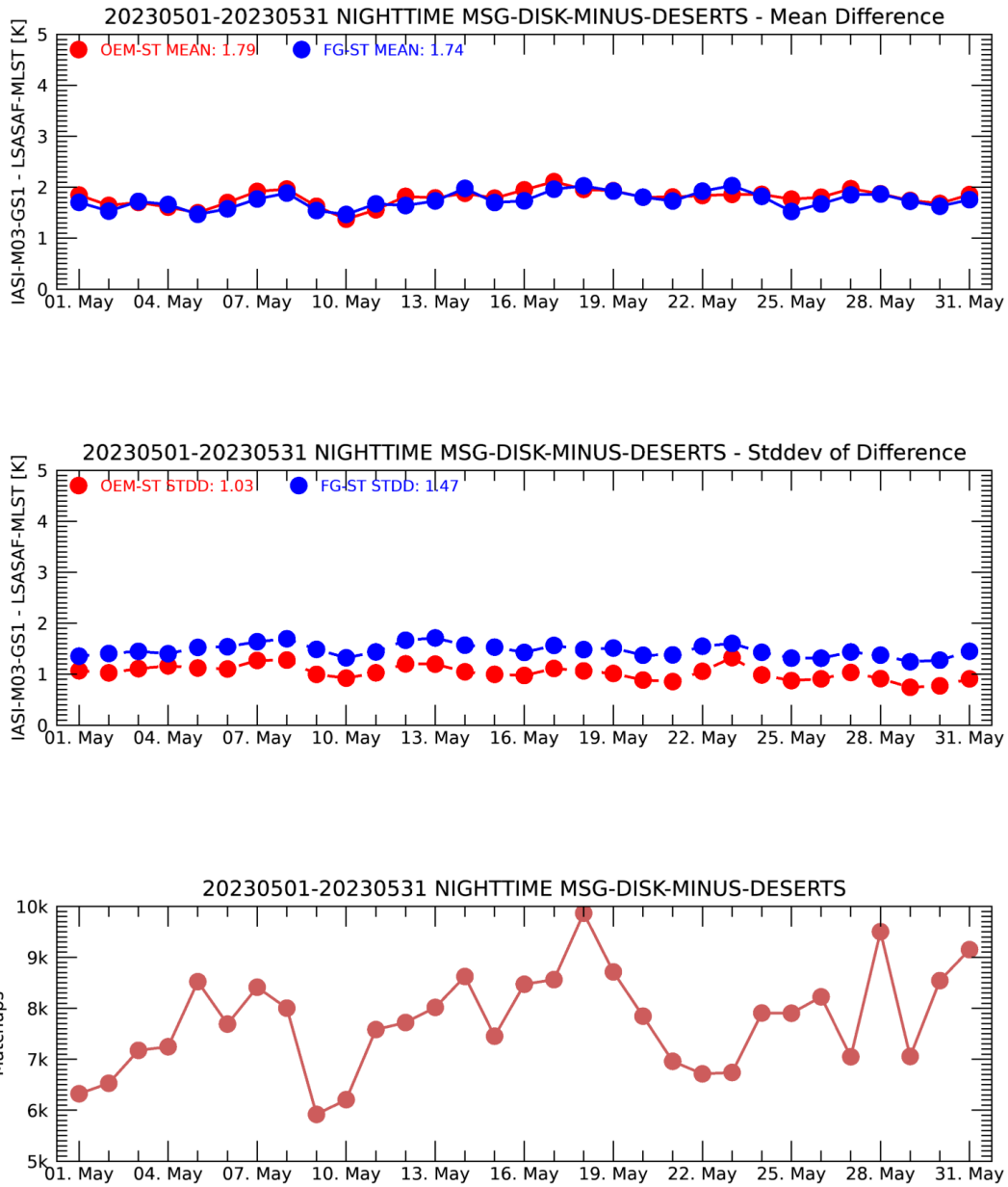
Figure 3.2: Monthly time series of mean difference and standard deviation between IASI L2 - LSA SAF. The bottom panel shows the number of daily match-ups. Nighttime statistics with M03 IASI L2 from GS1 for 01-31/05/2023
