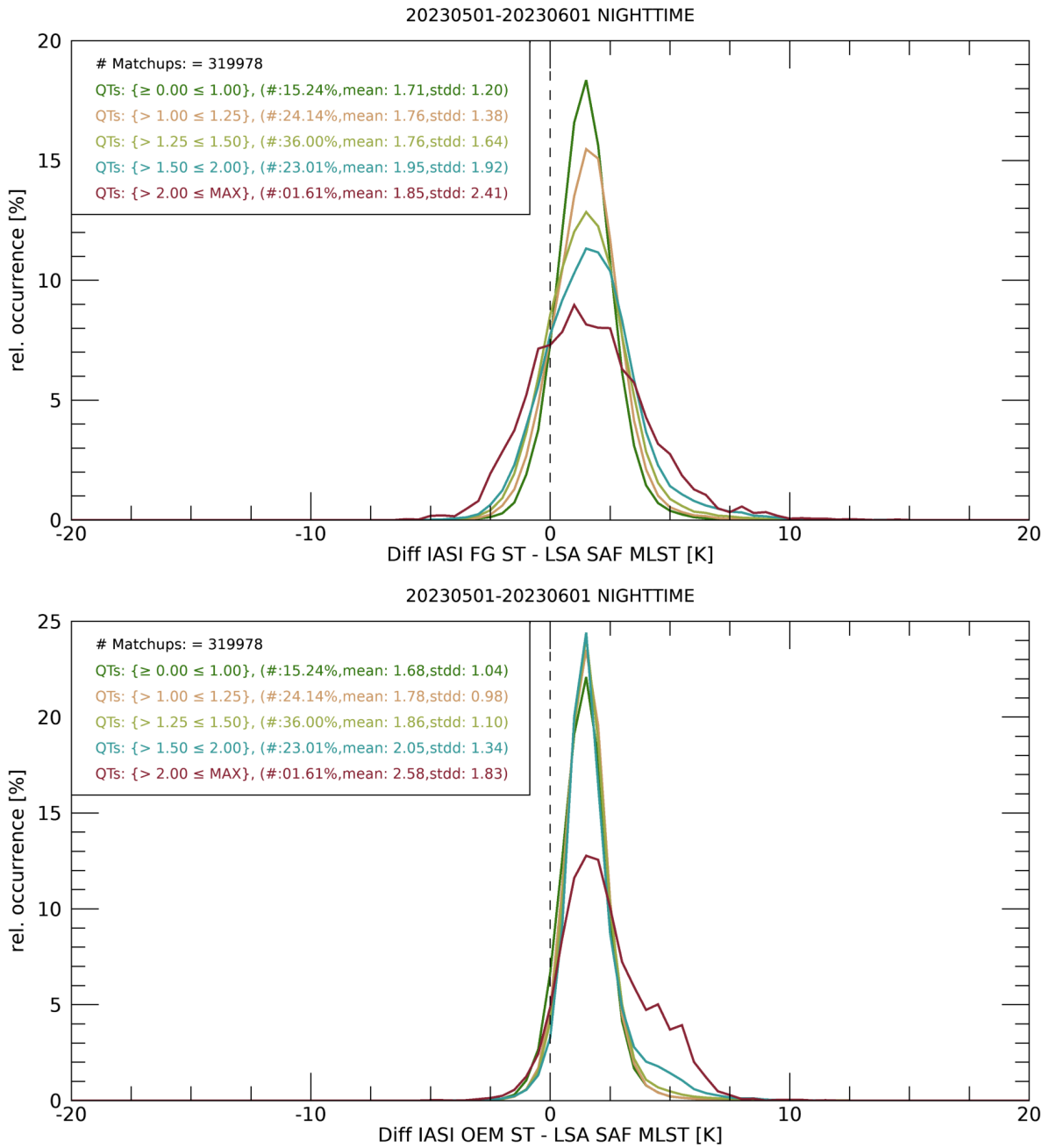
Figure 3.8: Difference histograms for different quality indicators for Regression (FG) (top) and OEM retrieval (bottom) retrieval between IASI L2 - LSA SAF, Nighttime statistics with M03 IASI L2 from GS1 for 01-31/05/2023
