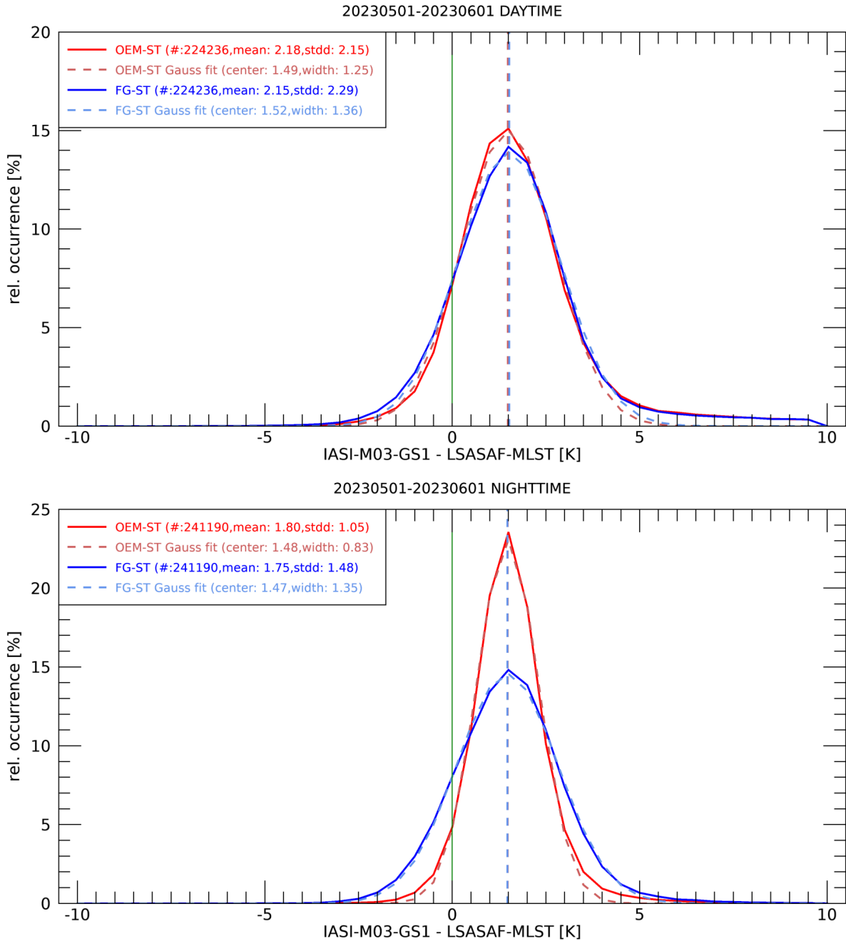
Figure 3.5: Daytime (top) and Nighttime (bottom) histogram of the difference between IASI L2 - LSA SAF, with M03 IASI L2 from GS1 for 01-31/05/2023
