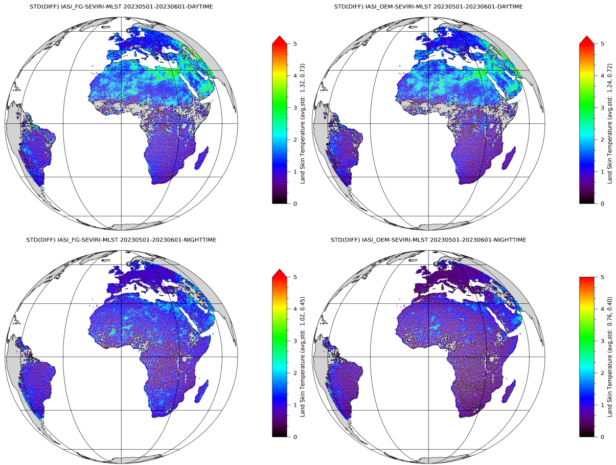
Figure 4.2: Day (top) and Night (bottom) Maps with the standard deviation of the differences IASI - LSA SAF for Regression (FG) (left) and OEM (right) retrieval, with M03 IASI L2 from GS1 for 01-31/05/2023
