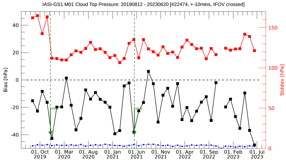
Figure 2.13: Long-Term Cloud Top Pressure Time Serie Bias and Standard Deviation of the differences, including fractional number of matchups per month (bottom blue) and #total-number-of-matchups (title). Global statistics with M01 IASI L2 from GS1.
