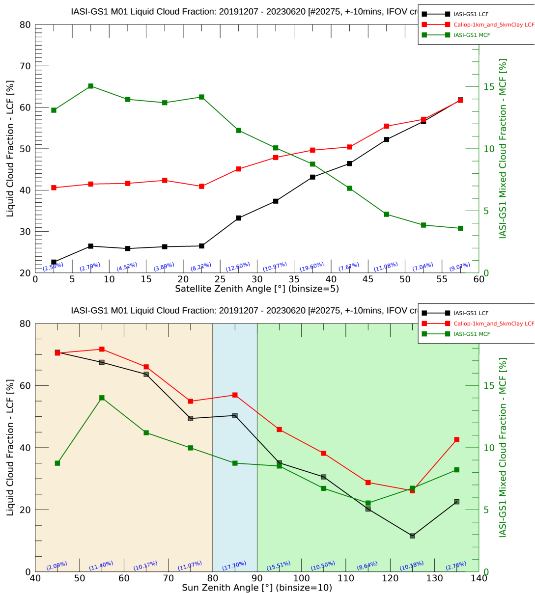
Figure 2.10: Satellite Zenith Angle (top) and Sun Zenith Angle (bottom) dependencies on Liquid and Mixed Cloud Fraction for IASI L2 and Caliop, Global statistics with M01 IASI L2 from GS1
