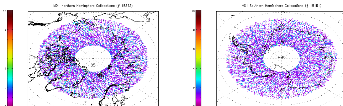
Figure 1.2: Northern (left) and southern hemisphere (right) matchups between Metop-B and Calipso! Due to different orbits the matchups within 10 mins are only possible at higher latitudes.
