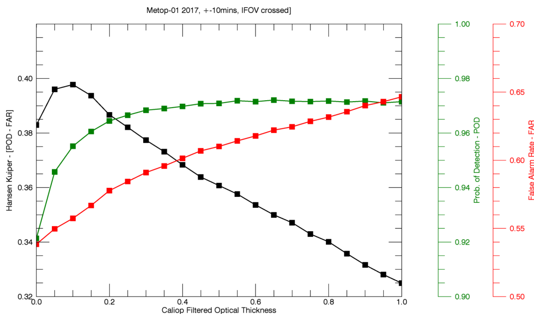
Figure 1.1: Hanssen Kuiper's skill Score, False Alarm Rate and Probability Of Detection as function of the filtered optical thickness (sum of the Calipso layer optical thickness).
