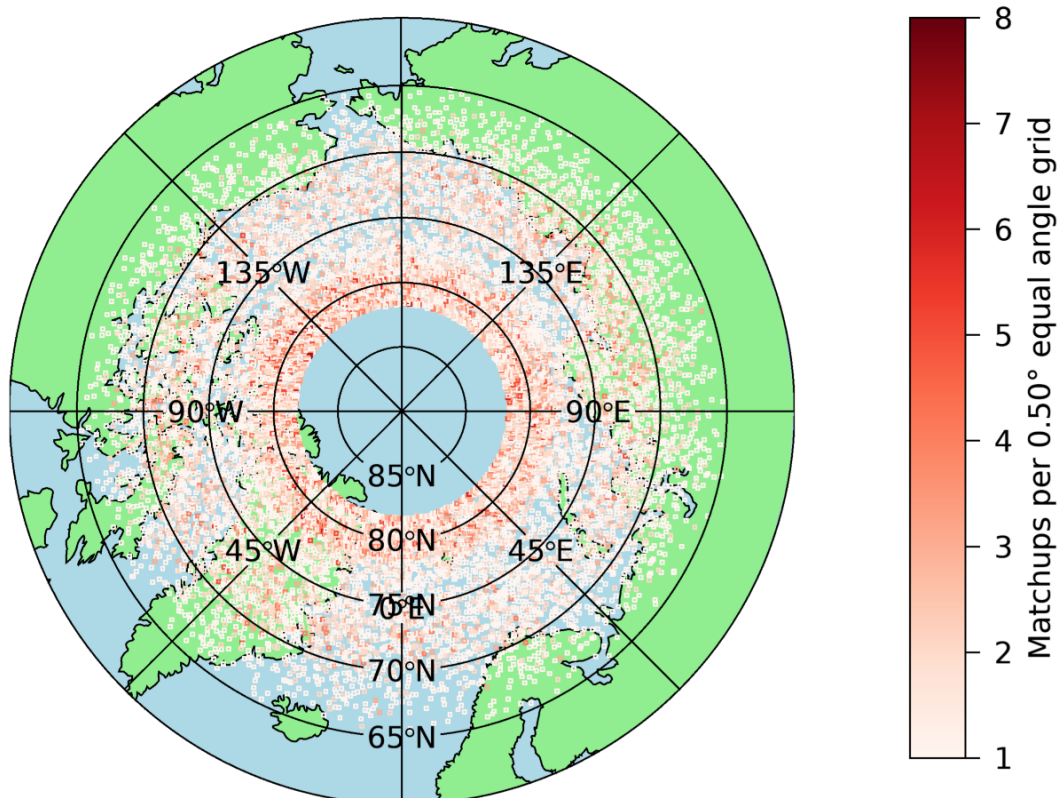
Figure 3.1: Northern Hemisphere Matchups between Calipso and M01 IASI L2 from GS1
