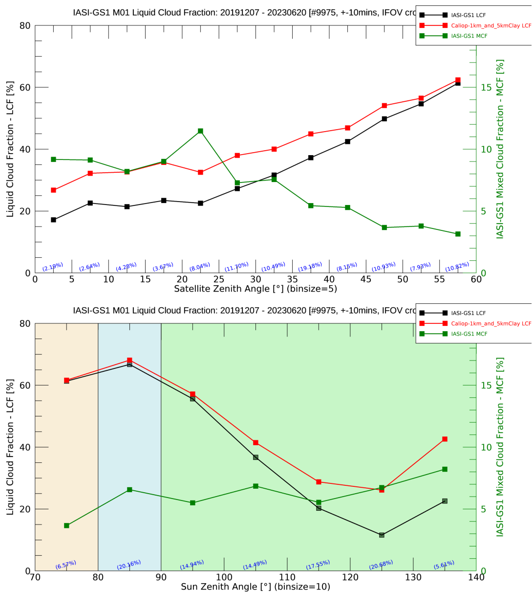
Figure 4.10: Satellite Zenith Angle (top) and Sun Zenith Angle (bottom) dependencies on Liquid and Mixed Cloud Fraction for IASI L2 and Calipso, Southern Hemisphere statistics with M01 IASI L2 from GS1
