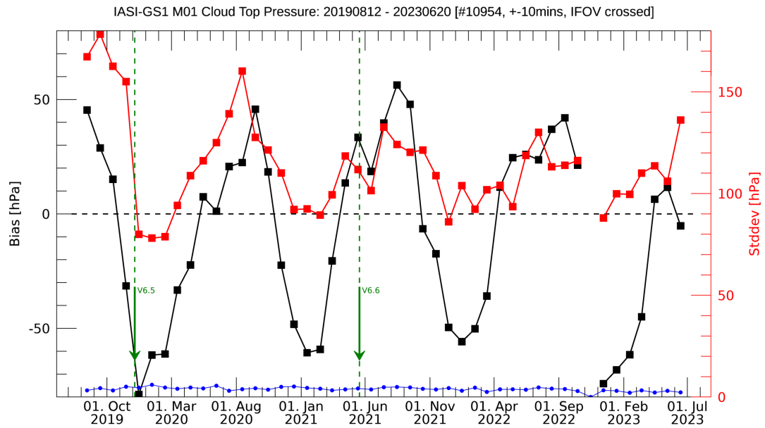
Figure 4.13: Long-Term Cloud Top Pressure Time Serie Bias and Standard Deviation of the differences, including fractional number of matchups per month (bottom blue) and #total-number-of-matchups (title). Southern Hemisphere statistics with M01 IASI L2 from GS1.
