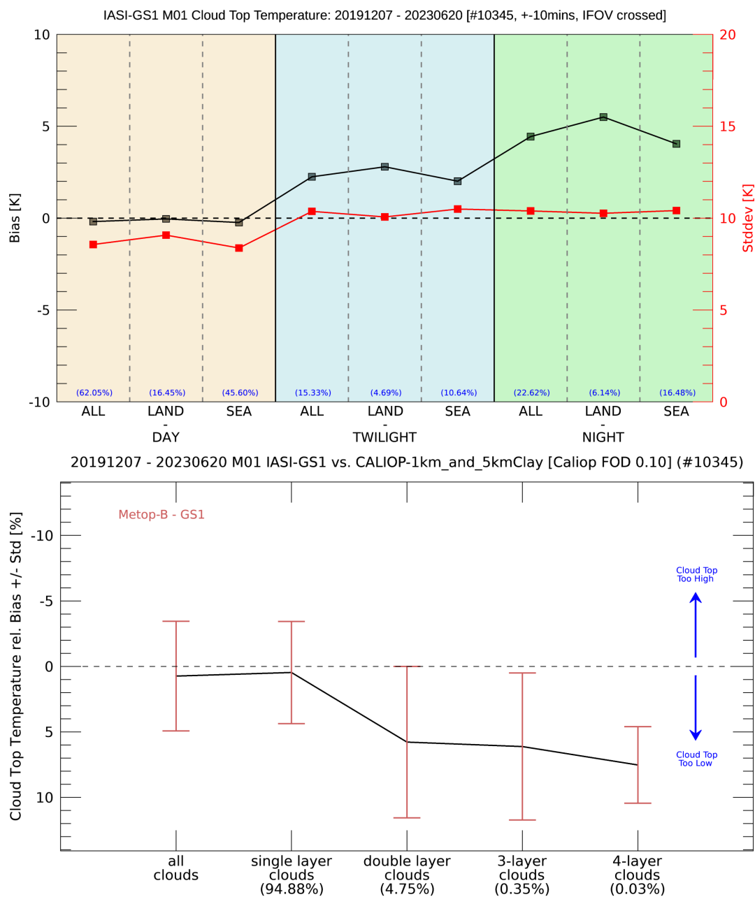
Figure 3.19: Cloud Top Temperature dependencies on Daytime/Land/Sea (top) and number of Calioop Cloud layer (bottom) between IASI L2 and Calioop, Northern Hemisphere statistics with M01 IASI L2 from GS1
