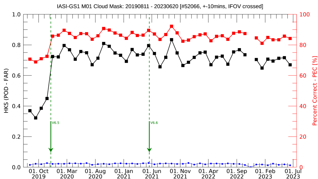
Figure 2.3: Long-Term Cloud Mask Time Serie for Hanssen Kuiper’s skill score and Percent Correct, including fractional number of matchups per month (bottom blue) and #total-number-of-matchups (title). Global statistics with M01 IASI L2 from GS1.
